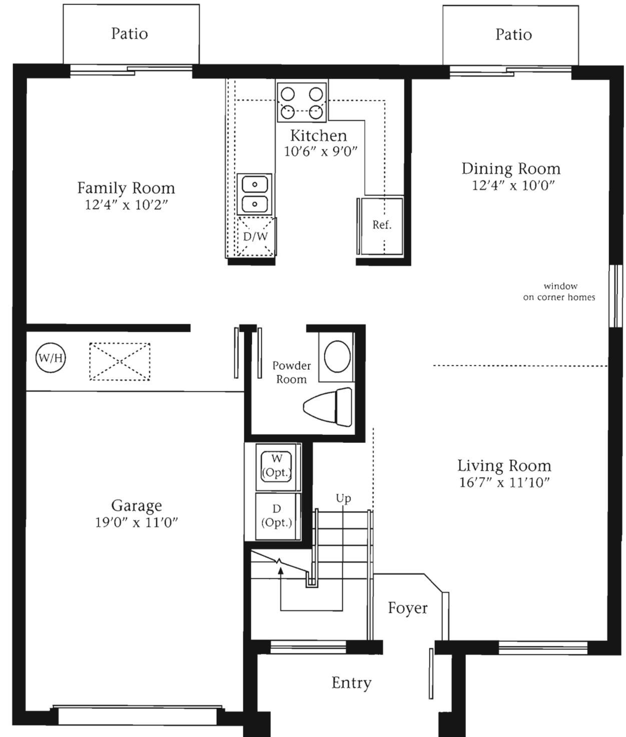
FIRST FLOOR
